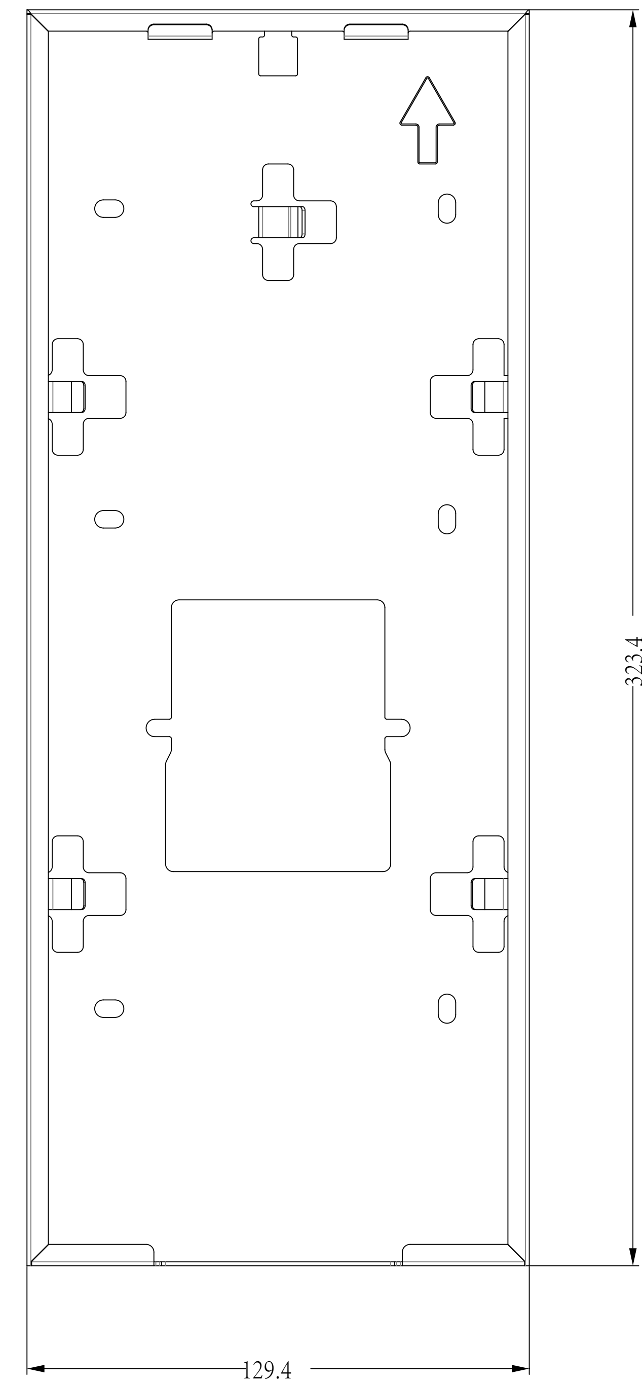
1 FRONT VIEW
