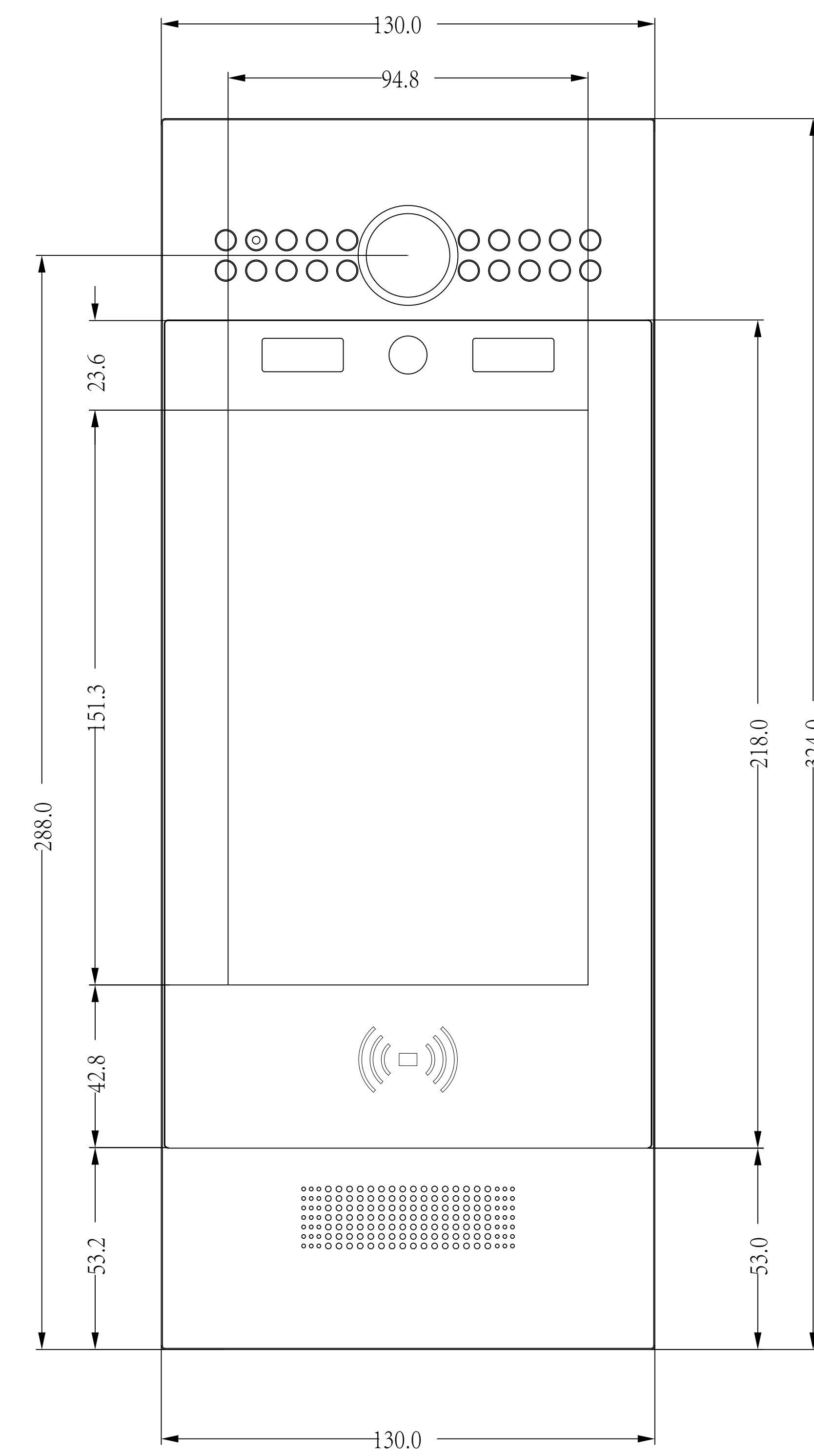
1 FRONT VIEW
