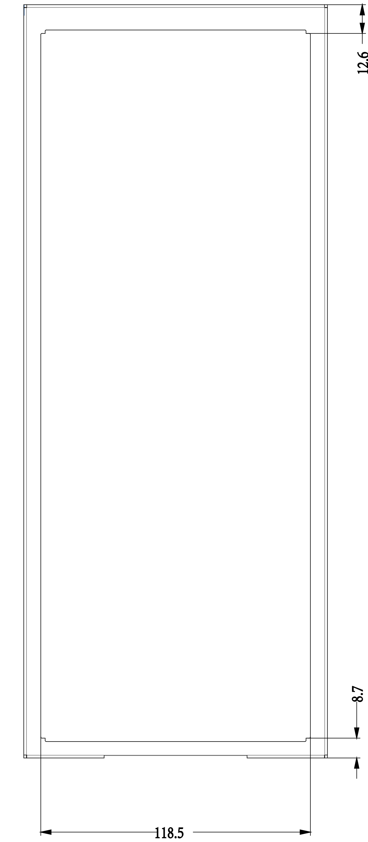
④ BACK VIEW
