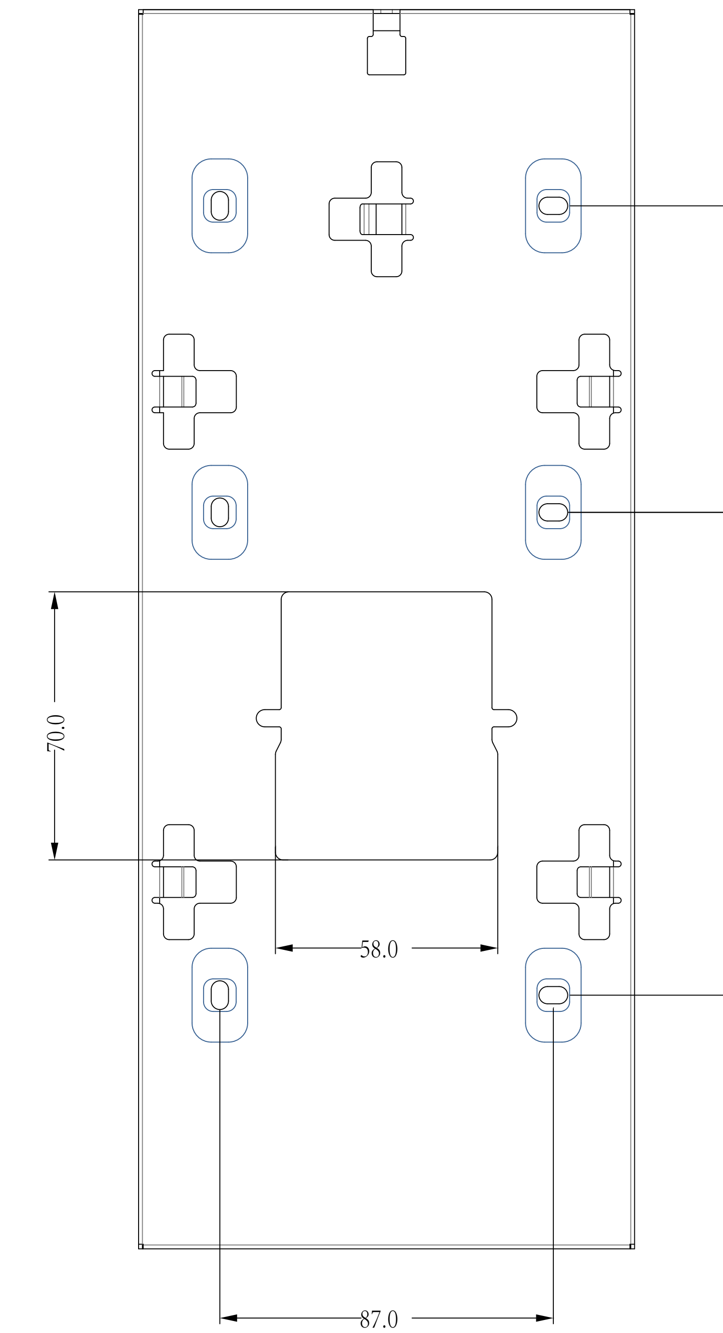
4 BACK VIEW
