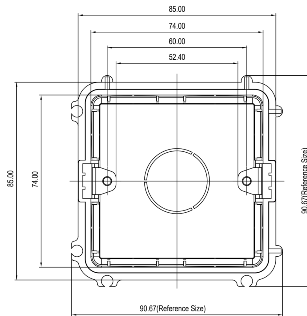
1 FRONT VIEW
